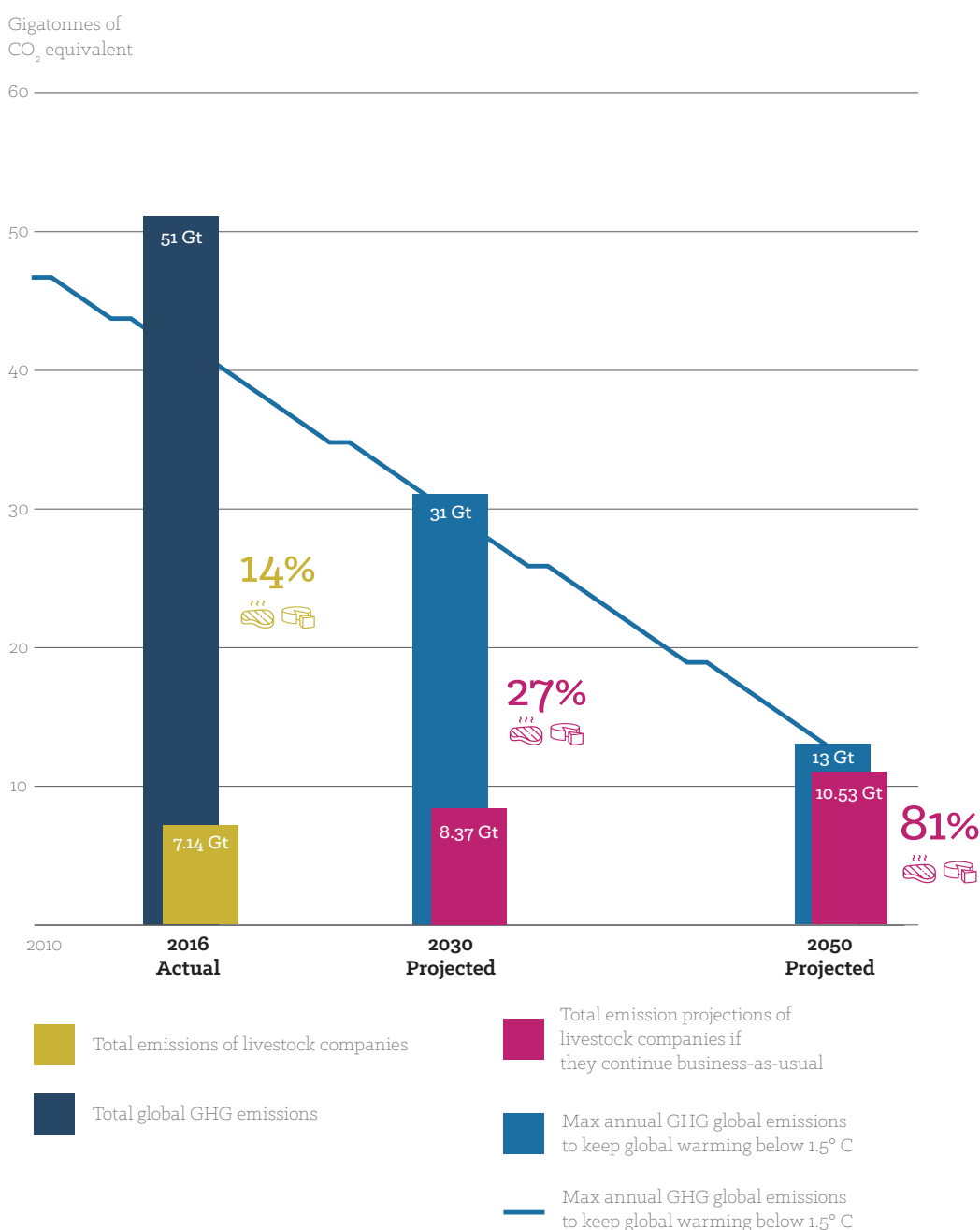
FIGURE 1: Estimated global greenhouse gas emission (GHG) targets to keep within a 1.5°C rise in temperature compared to emissions from global meat and dairy production based on business-as-usual growth projections.
